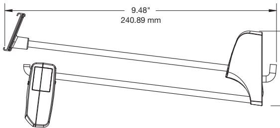
IR StopLok™ with Flexible Locking Hook - Double Wire 9", American Pegboard (NF2LOK9):
