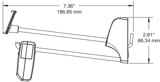
IR StopLok™ with Flexible Locking Hook - Double Wire 7", European Pegboard (NF2LOK7E):
