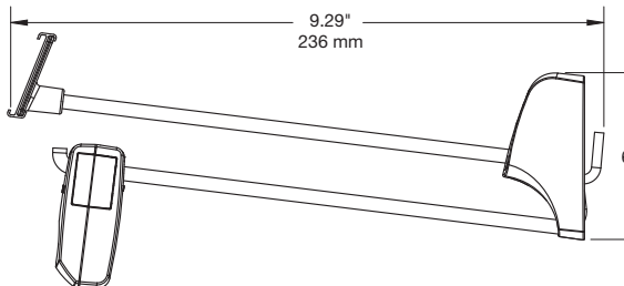
IR StopLok™ with Flexible Locking Hook - Double Wire 9", European Pegboard (NF2LOK9E):
